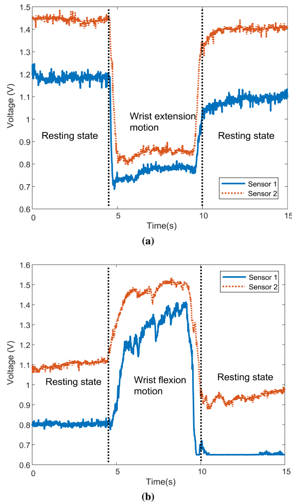
Fig. 5 Measured signals from bracelet sensor: (a) signals from wrist extension motion, (b) signals from wrist flexion motion.
