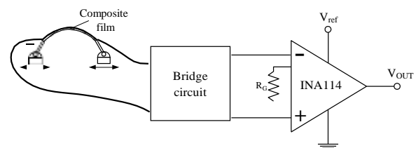
Fig. 4 Transducer circuit of bracelet sensor
