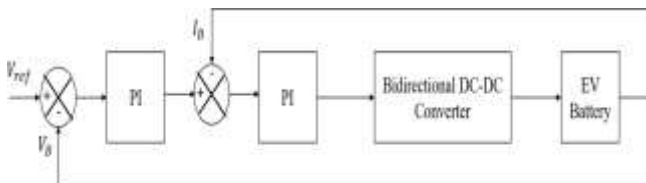
Fig.4. Closed loop control circuit for bidirectional DC-D Converter.
