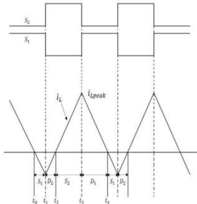
Fig.3.Gatedrivers for switches and diodes.
