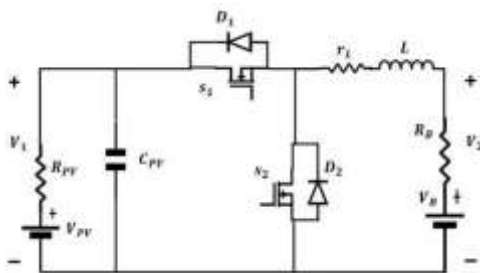
Fig.2.Bidirectional DC-DC converter.
