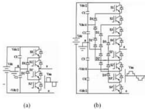
Fig:2 Topology of the diode-clamped inverter (a)
