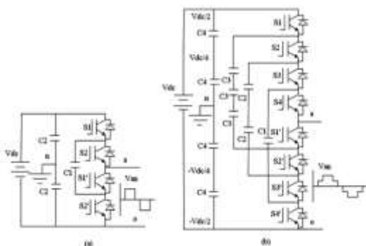
Fig:3 Capacitor-clamped multilevel inverter circuit
