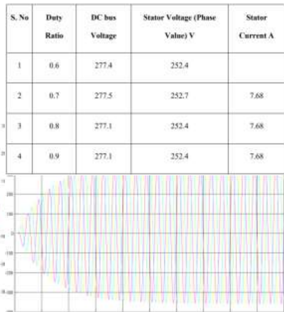
Fig 10: Steady state values of stator current and applied voltages of Induction motor.
