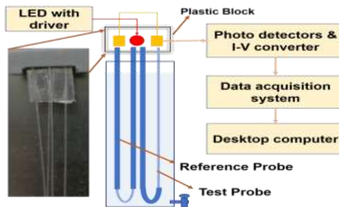
Figure 1. Schematic showing block diagram of experimental setup consists of two U-bent POEs (decladded region of fiber represented as a thin line) dipped in a 55 cm long liquid column, home-made plastic block to house LED and PDs, optoelectronic circuitry, and DAQ.
