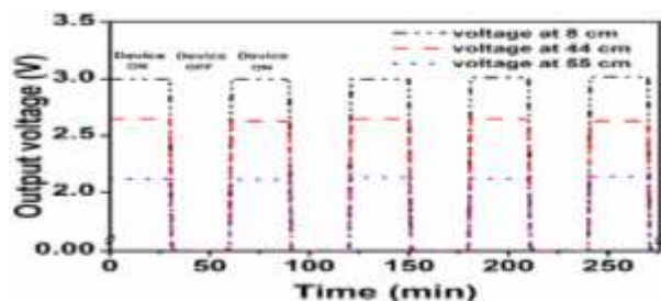
Figure 5. Temporal response of the sensor over four hours indicating a stable response. The sensor was switched 'ON' for 30 min and then switched 'OFF' for the next 30 min at different liquid levels.
