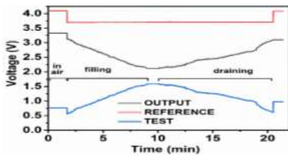
Figure 2. (a) Sensor response recorded in terms of voltage while the 60 cm long glass column is continuously filled and drained with water over time of 20 min.
