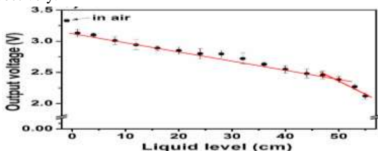
Figure 2. c) The relationship between output voltage and the liquid level.
