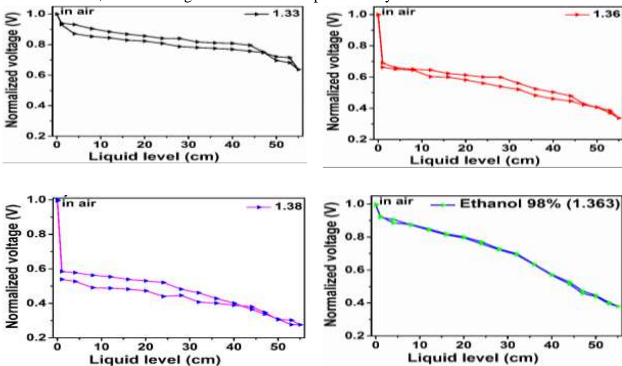
Figure 3. Normalized differential voltage response from the fiberoptic level sensor subjected to filling and draining of liquids of different refractive index values including salt solutions of RI (a) 1.33 (no salt), (b) 1.36 and (c) 1.38 as well as (d) ethanol 98% with RI value of 1.363.
