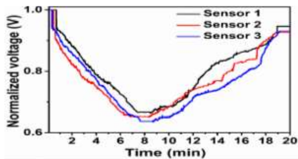
Figure 2. (b) Normalized voltage response from three different test probes over time.
