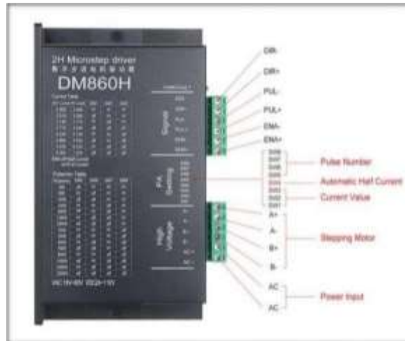
Fig 5.4 Driver module
