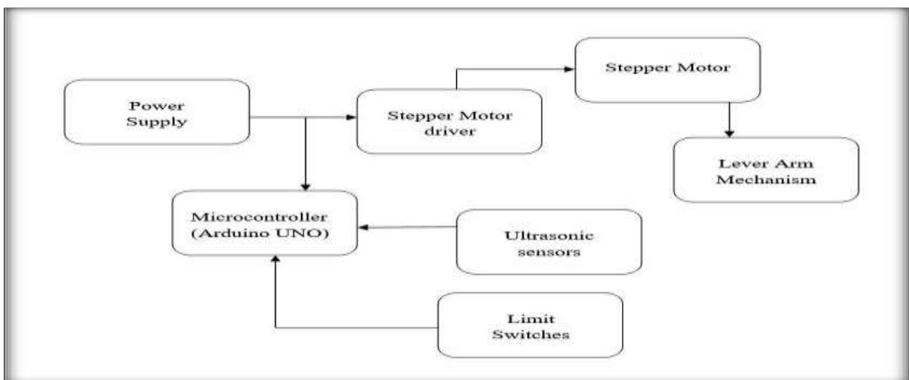
Fig. 3.1 Block Diagram
