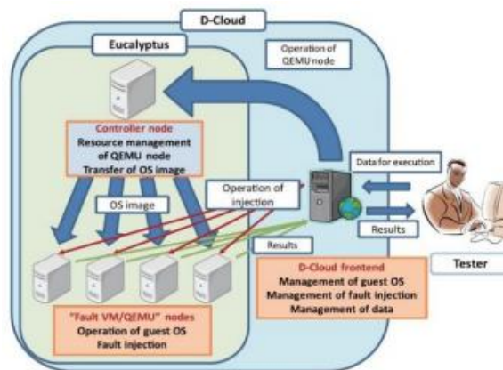
Fig. 5 Architecture of D-Cloud
