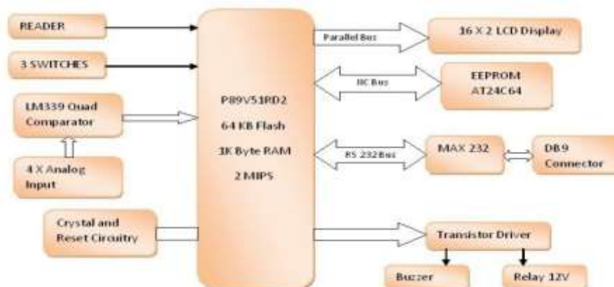
Figure 2. Block Diagram of Microcontroller and Associated Circuitry
