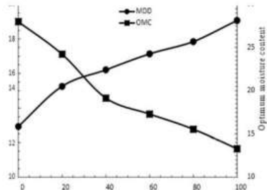
Figure 6 variation of OMC and MDD with addition of Campus soil to dredged soil
