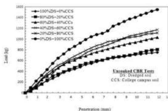
Figure 9 Load penetration curves for dredged soil (unsoaked condition)
