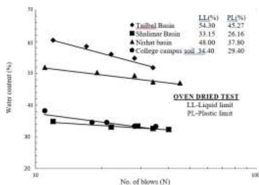
Figure 4 flow curves of oven dried samples
