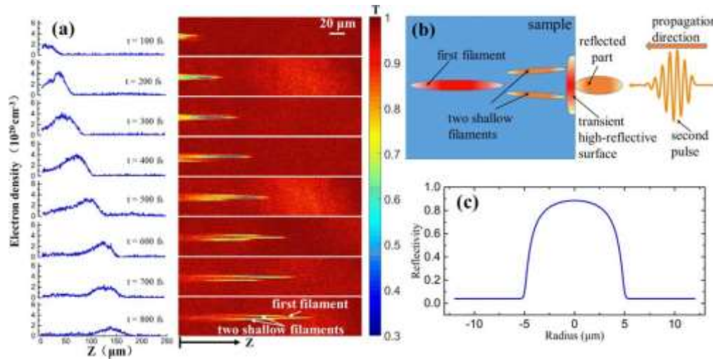
Figure 2. (a) Two-dimensional transmission mapping and electron density evolution at the centers of filaments induced by double pulses with t = 200 \text{ fs} . The energy of both pulses was 4 \mu\text{J} . T denotes the transmissivity. (b) Diagram of the filament split caused by the highly reflective surface induced by the first pulse. (c) Instantaneous reflectivity of the surface at a delay of t = 200 \text{ fs} from simulation. Reproduced from [38]. © 2019 The Japan Society of Applied Physics. All rights reserved.
