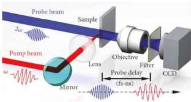
Figure 1. Schematic of the time-resolved pump-probe shadowgraphy setup. Reproduced from [30]. CC BY 4.0.
