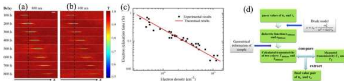
Figure 5. Time-resolved transmissivities of the femtosecond-laser-induced region in fused silica with (a) 800 nm and (b) 400 nm probe pulses at delay times of 100–800 fs. The pump pulses of both (a) and (b) propagate from left to right. The color map is selected to enhance transmissivity changes and plasma evolution after laser pulse irradiation. The scale bar is 20 \mu\text{m} . The black lines with arrows denote the propagation direction of the pump pulses. (c) Evolution of the electron relaxation time with the electron density. The black squares denote the measured pairs of n_e and \tau_e . The red solid line represents the theoretical results obtained using the electron-ion scattering equation. (d) Schematic of the method for determining the dielectric function. Reprinted from [45], with the permission of AIP Publishing.
