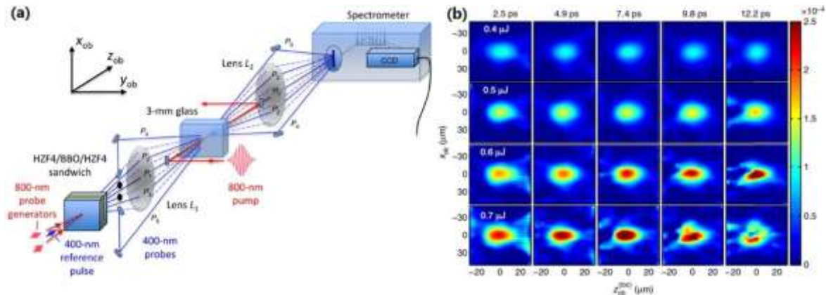
Figure 18. (a) Schematic of the SFDT system based on angle division. (b) Imaging of the nonlinear index profile at four different pump energies and five different propagation times. Reprinted by permission from Macmillan Publishers Ltd: Nature Communications [83], Copyright 2014.
