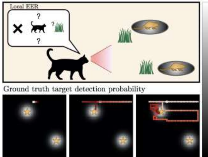
Figure 7: Infotaxis : Upper panel: A cat searches for the two yellow mice. The distribution around the mice represents the probability of detecting the mouse at that location where white is high probability. The gradient in the cone around the cat represents the cat's measurement model. The cat has a mental image of the expected local reduction in entropy for moving up, down, left or right. Lower panel: This is an example of an infotactic trajectory of an agent searching for target locations, represented by the yellow stars. The likelihood of detecting the target is represented by the distribution around the target locations, becoming more dense closer to the target. The measurement model encodes the ability of a camera to detect an object at a particular range and angle of attack. The search strategy selects the direction of movement that maximizes the expected entropy reduction at each time step. The infotaxis strategy succeeds at finding
