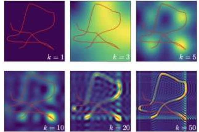
Figure 6: Fourier transform of a trajectory: The Fourier transform of a constant speed trajectory represents the trajectory in the form of a spatial distribution. The representation of the trajectory by its transform changes in granularity for k = 1, 3, 5, 10, 20, 50 Fourier coefficients.
