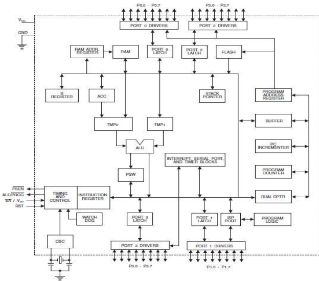
FIG. 4. . BLOCK DIAGRAM OF MC AT89S52 XII. MICROPROCESSOR AT89S52
