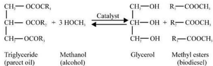
Fig 1. Transesterification reaction
