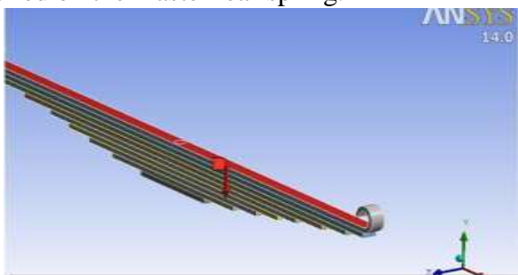
Fig. 7 - Loading Condition
