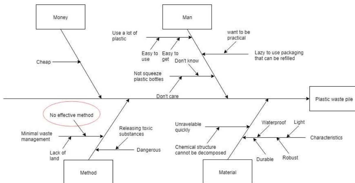
Figure 12. Fishbone diagram.
