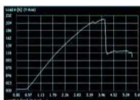
Graph 5.3 Flexural test on 4 Specimen
