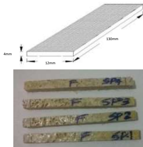
Fig 4.2 Flexural test specimens
