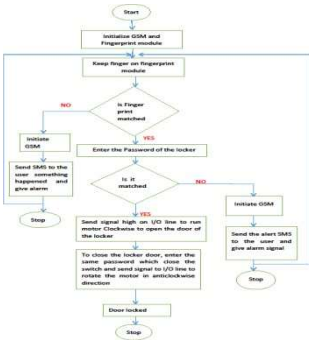
Figure 8. Flow chart for Fingerprint and Soft password based Home Locker Security System using GSM Modem
