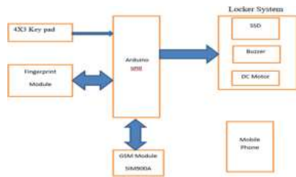
Figure 1. Block diagram of Advanced Alert Home locker security system.
