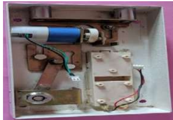
Figure 4 (b). Electro mechanical Motor arrangement
