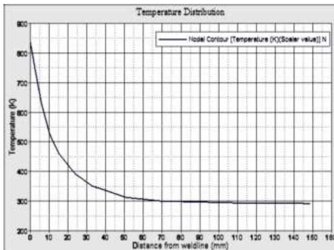
Fig.10 Temperature distribution for advancing side during Transient finite element analysis of friction stir welding an tool as a steady state heat source in mid of the plates.
