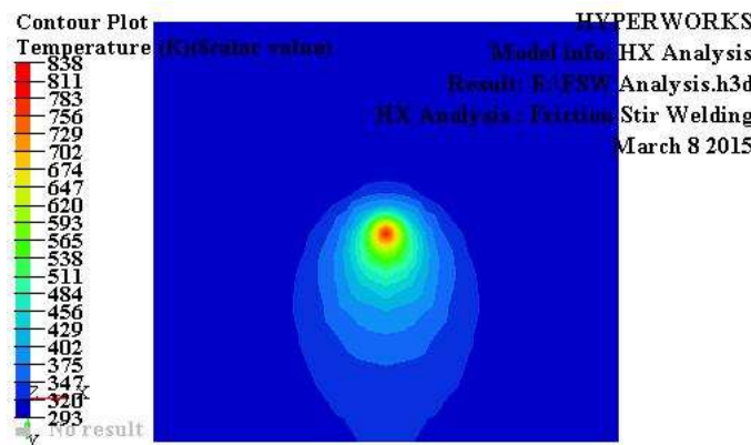
Fig. 8 Temperature distribution from top surface of the workpiece.
