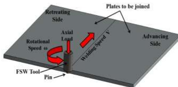
Fig.1 The schematic model of friction stir welding
