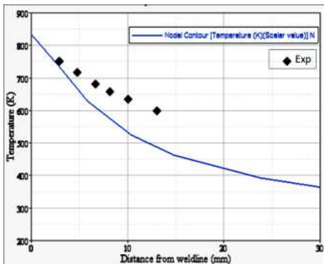
Fig. 11 Comparison of Simulated temperature and experimental maximum temperature as a function of distance from weldline.
